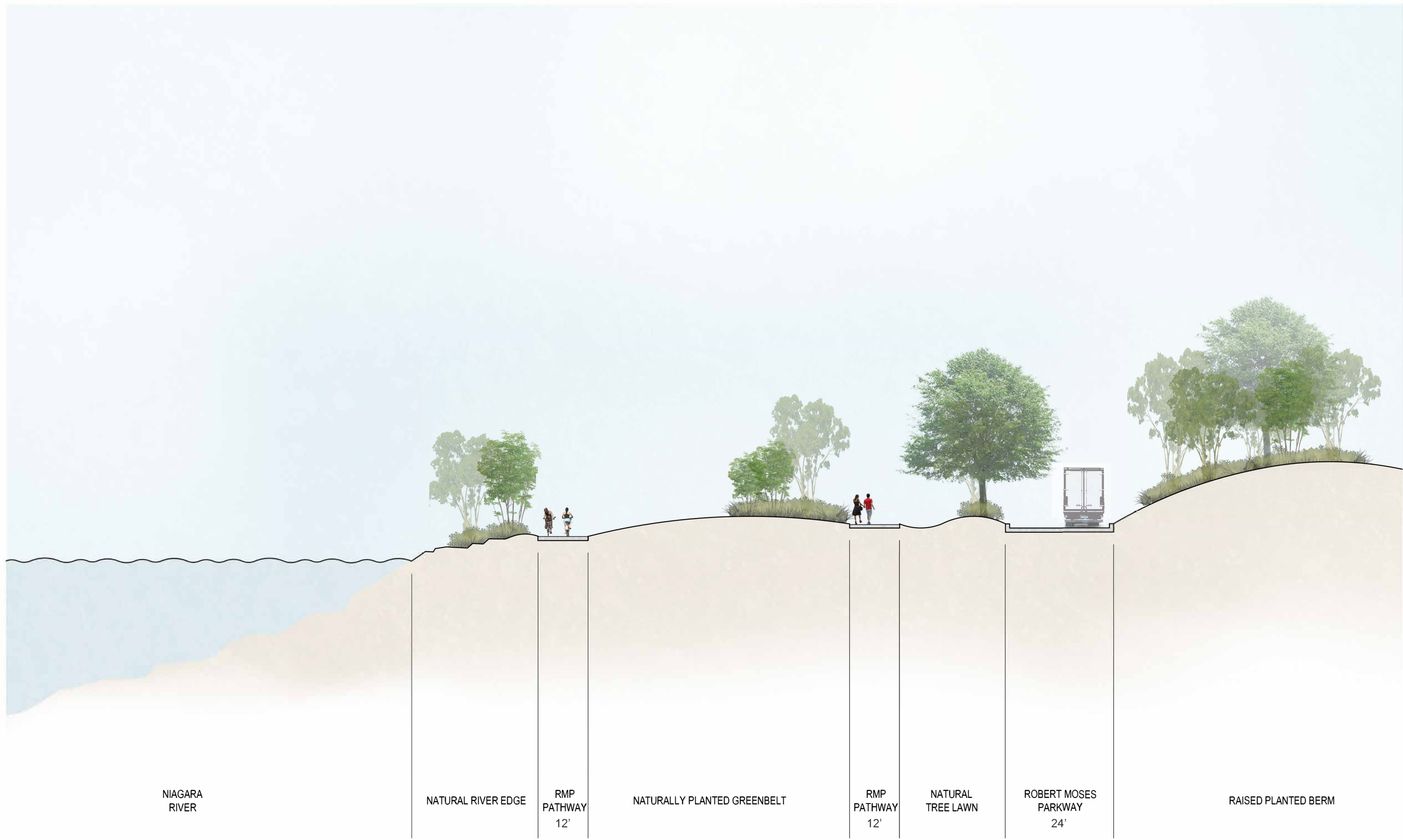
ROBERT MOSES PARKWAY: MULTI-USE TRAIL - TYPICAL SECTION
